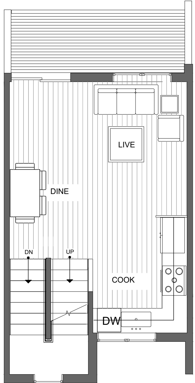
SECOND FLOOR
