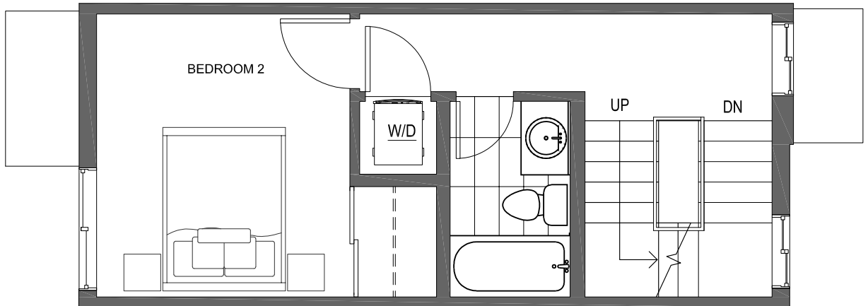
SECOND FLOOR
