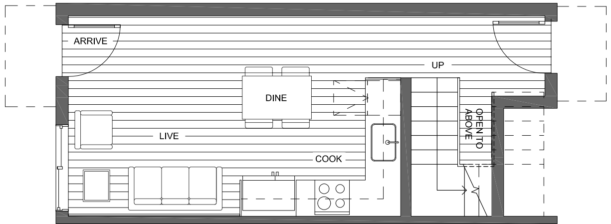
FIRST FLOOR
