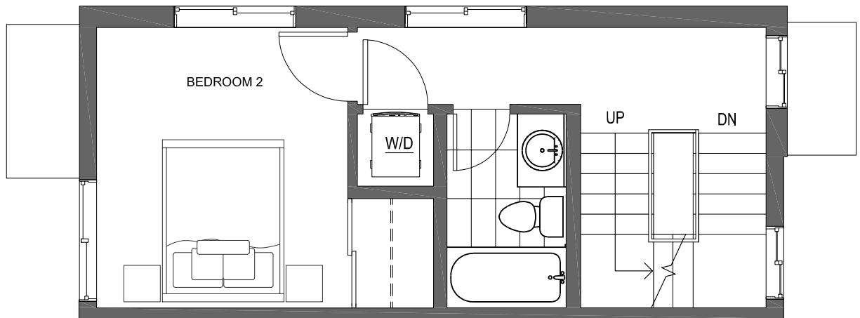
SECOND FLOOR
